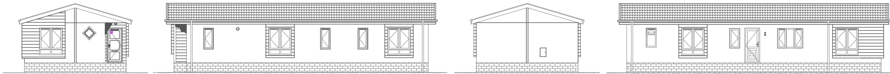
(C) Elevation - Front
