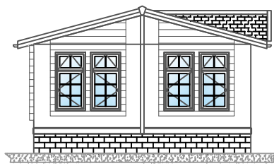
Elevation C
